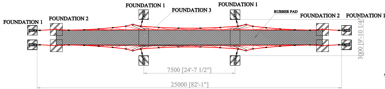
LAYOUT DRAWING
