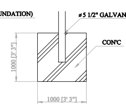
FOUNDATION 2 DETAIL (SIDE VIEW)
