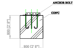
FOUNDATION 2 DETAIL (SIDE VIEW)
