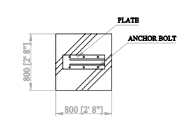
FOUNDATION 2 DETAIL (PLAN)
